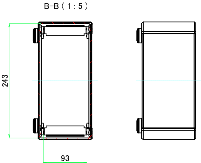
D view
