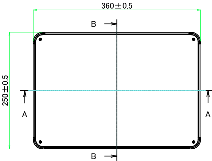
E view
